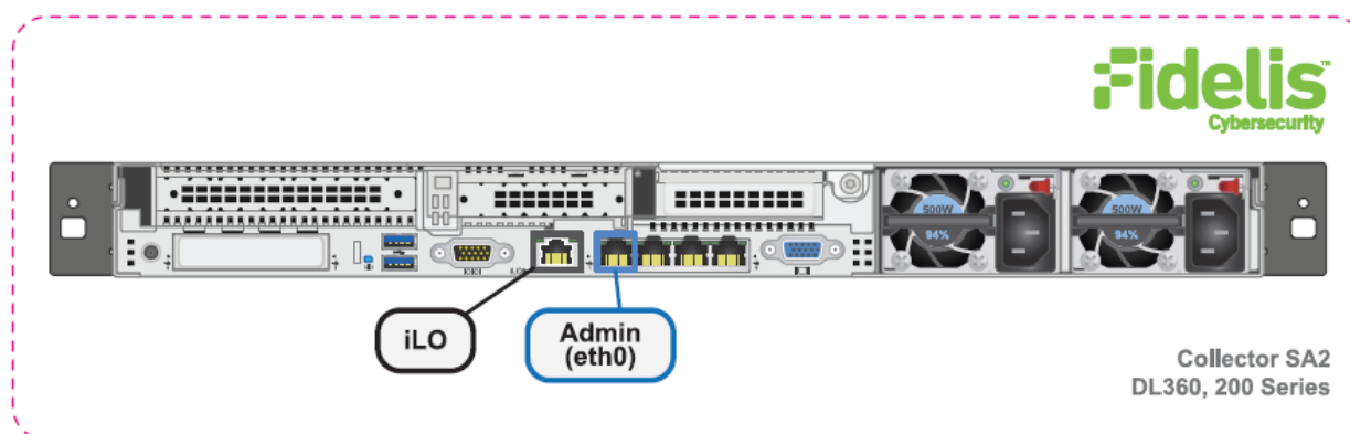
Figure 3: Network Port Assignments — Collector SA (Rev-J)
